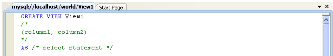
Figure 20.13. Editing View SQL
